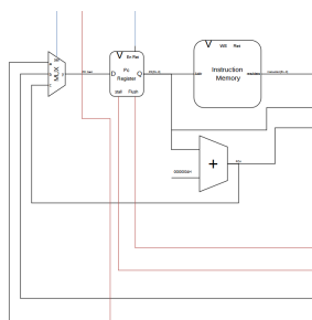
Figure 2.3: RV32ICore IF Stage
